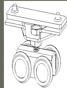
TOP ROLLER ASSEMBLY (SURFACE HUNG DOORS AND POCKET DOORS)
